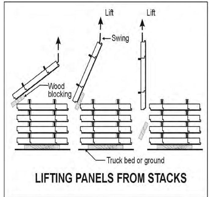
Figure 14: Lifting panels from a stack.
