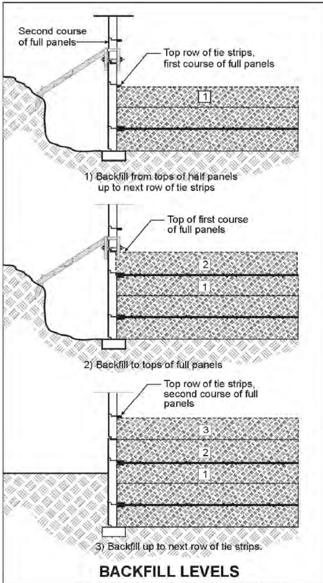
Figure 31: Backfill levels.
