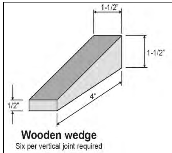
Figure 4: Wooden wedge.
