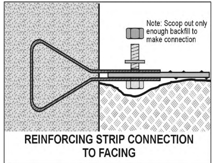
Figure 28: Reinforcing strip connection to facing.
