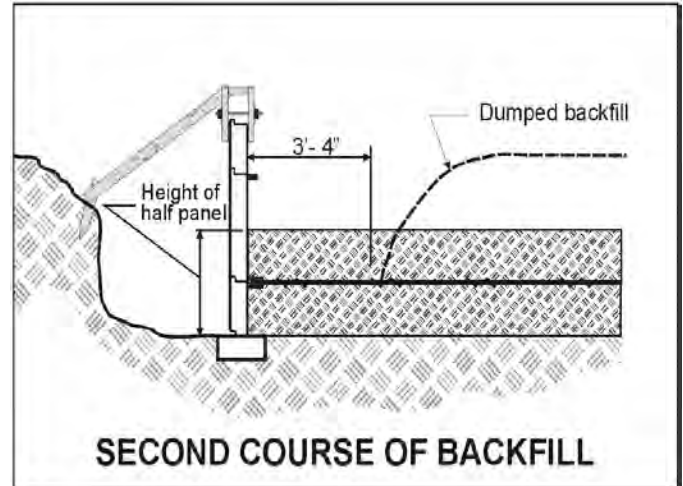
Figure 27: Second course of backfill.
