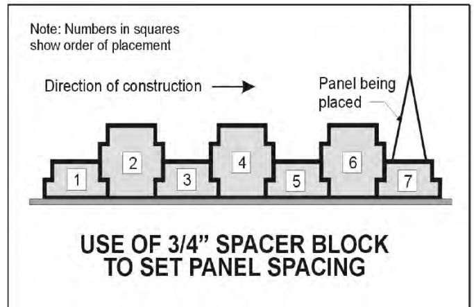
Figure 15: Use of spacer block to set panel spacing.
