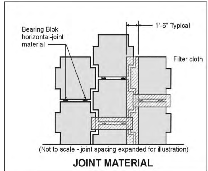
Figure 24: Joint material.
