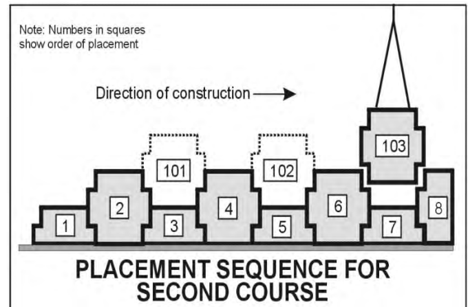
Figure 30: Placement sequence for second course.
