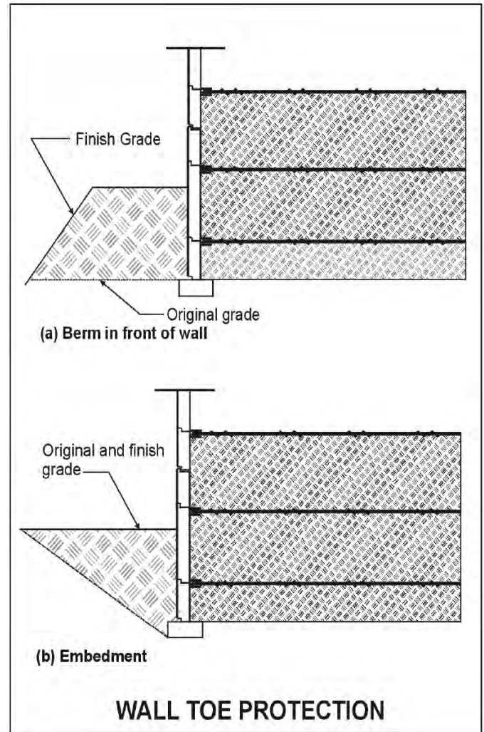
Figure 32: Wall toe protection.
