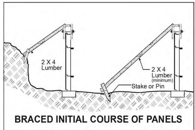
Figure 23: Panel bracing
